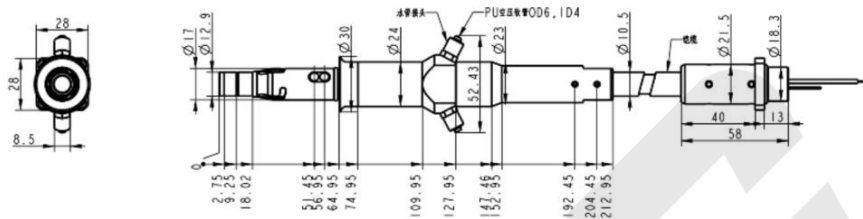
Outline dimension drawing of laser output terminal (unit: mm)
